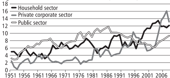
Figure 2: INDIA: INVESTMENT (% GDP)
